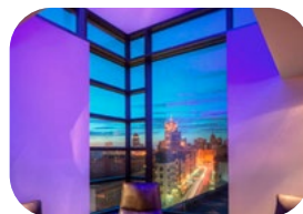
Ultraviolet (UV)
